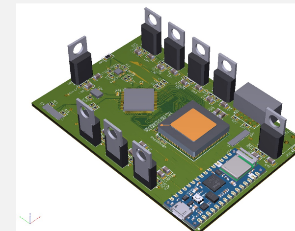
(Left) CAD of short-pulse board. (Right) Board for testing short-pulse locking algorithm.
