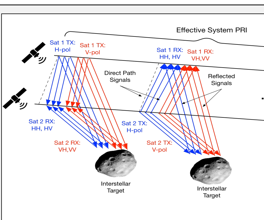
Pulse exchange, scheduling, and synchronization for quad-pol bistatic measurements.
