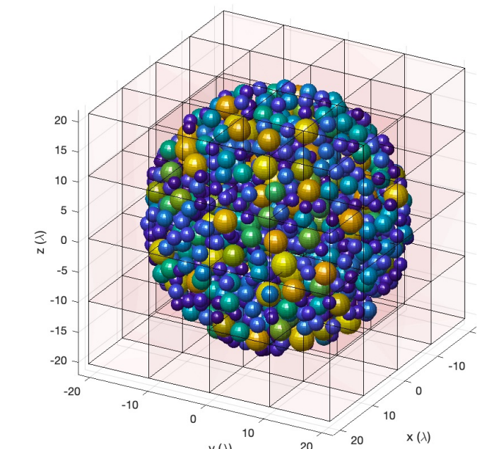
Adaptive Multi-level T-matrix Method for simulating scattering from electrical-large collections of objects.
