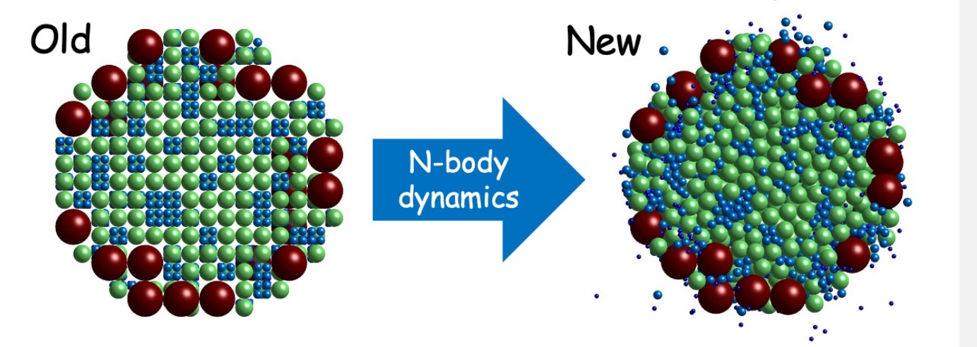
Asteroid rubble pile model generation using N-body gravitational dynamic settling.
