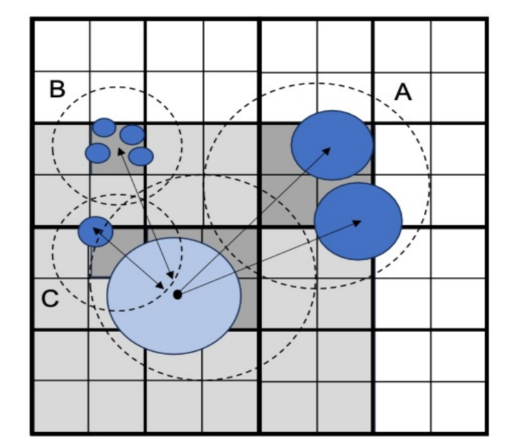
Adaptive Multi-level T-matrix Method for simulating scattering from electrical-large collections of objects.
