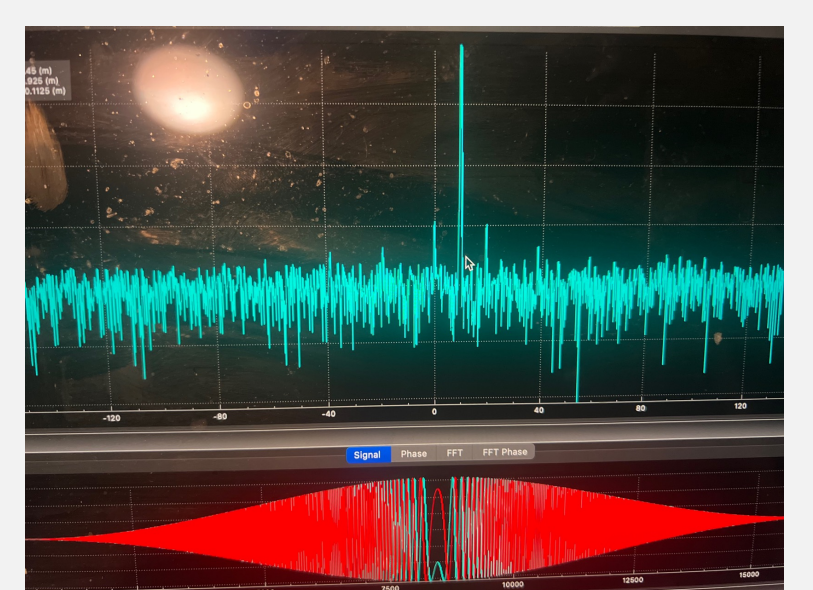
(Left) Digital test bed (COTS RF System on a Chip) for developing bistatic timing synchronization firmware. (Right) Range compressed pulse from SDRadar FPGA core.
